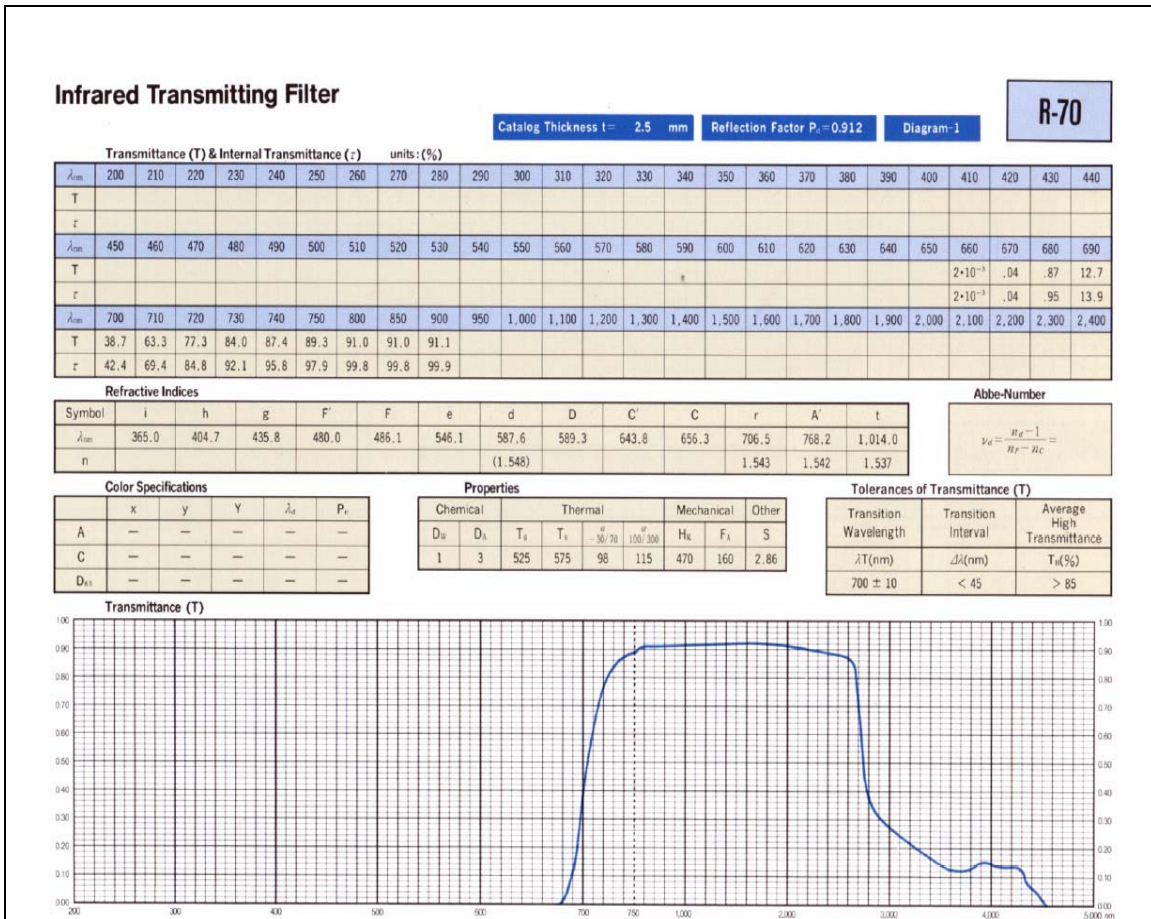
Figure 27. R-70 Infrared Transmitting Filter Curve
