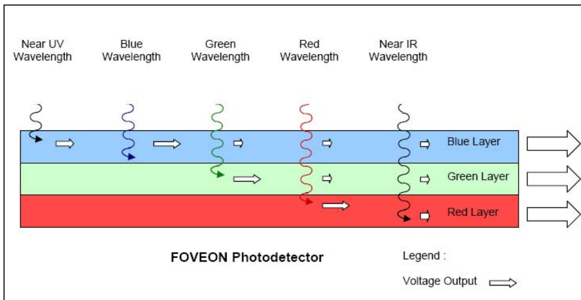
Figure 9. FOVEON camera absorption mechanism for various wavelengths [4].
