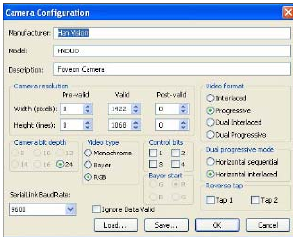
Figure 7. Frame-Grabber FOVEON Specification
